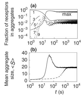
FIG. 4. Kinetics of the TLBR model. (a) Fraction of receptors in aggregates with 1, 3, 5, 7, or 9 receptors or in the largest aggregate as a function of time in the sol-gel coexistence phase ( N_L=50\,000 and c=2.7 ). (b) Mean aggregate size as a function of time for the same conditions as (a) (solid line) and at a lower ligand concentration (dashed line) that gives the same mean size at equilibrium ( N_L=2000 and c=0.11 ). Additional simulation parameters: N_R=3000 , \beta=16.8 , and k_{\text{off}}=0.01\text{ s}^{-1} . Results are averaged over 40 simulation runs. Mean aggregate size is determined by \langle S \rangle = \sum_{i=2}^{N_R} i n_i / \sum_{i=2}^{N_R} n_i , where n_i is the number of aggregates containing i receptors. Parameter values were chosen arbitrarily for the purpose of demonstrating the rule-based KMC method, but they are expected to be somewhat reasonable for the case of a population of ligands, each with three 2,4-dinitrophenol (DNP) hapten groups, interacting with a population of monoclonal cell-surface anti-DNP IgE antibodies, each with two antigen-combining sites [24,26].
